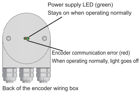
Back of the encoder wiring box
